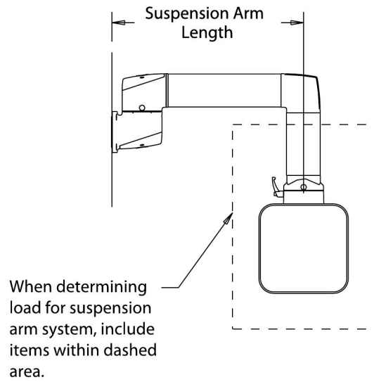
Load Diagram
